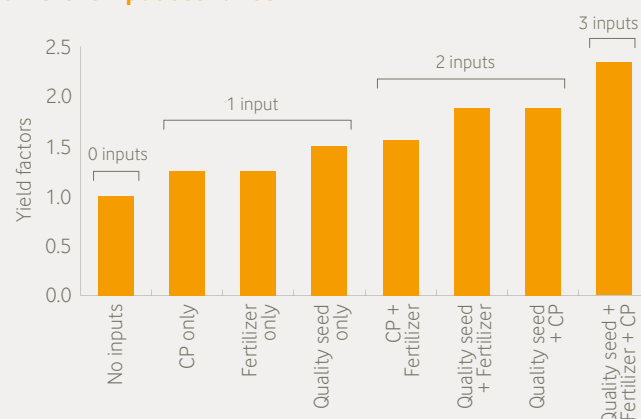
Figure 8: Schematic representation of yield under different input scenarios
